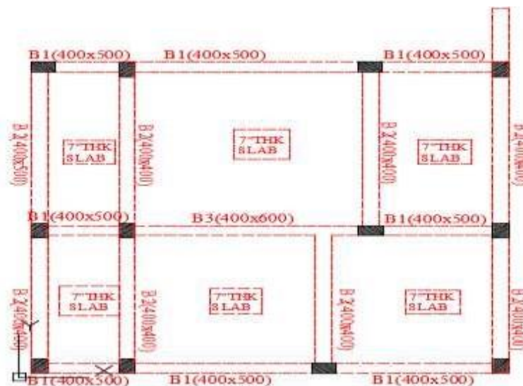
Fig-6: showing beam layout of the structure
